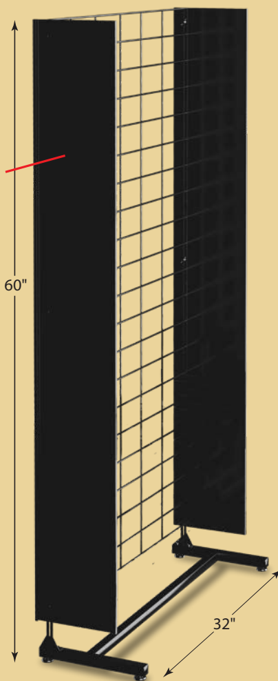
32" x 60" PowerGrid™ with 3" grid spacing With Casters PG-3260C-3-B With Levelers PG-3260L-3-B
