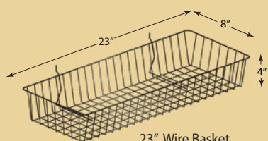
23" Wire Basket PGB-23X8X4-B
